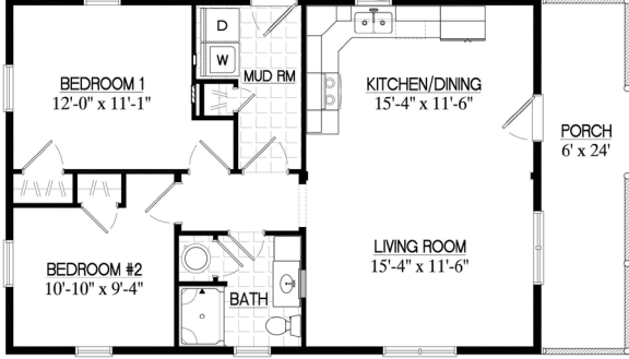
24SR402 24x36 Settler
